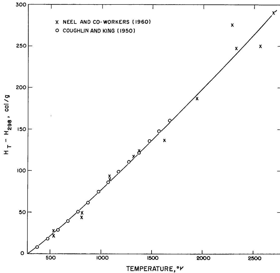
Figure II.1.5 Heat Content of ZrN as a Function of Temperature
