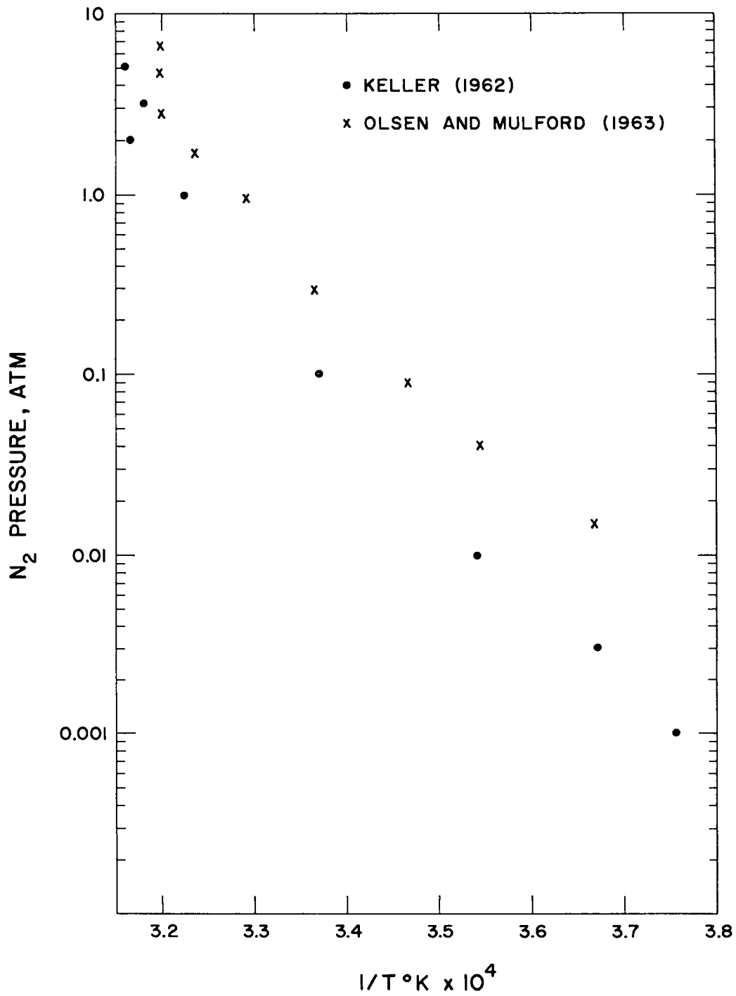
Figure III. 2. 2 The Melting Point of UN as a Function of Nitrogen Pressure
