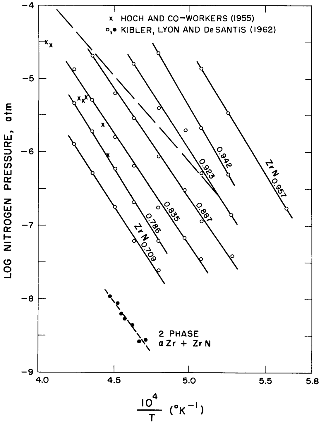
Figure II. 1.7 Pressure of Nitrogen over ZrN as a Function of 1/T
