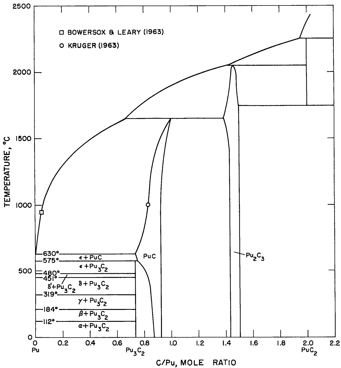
Figure III. 1.7 Tentative Phase Diagram of the Pu- Pu_3C_2 System
